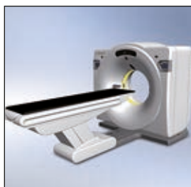
Wire-actuated encoders are the preferred solution in medical technology applications for adjusting the height or length of tomographs, operating tables, examination chairs and also x-ray equipment.
