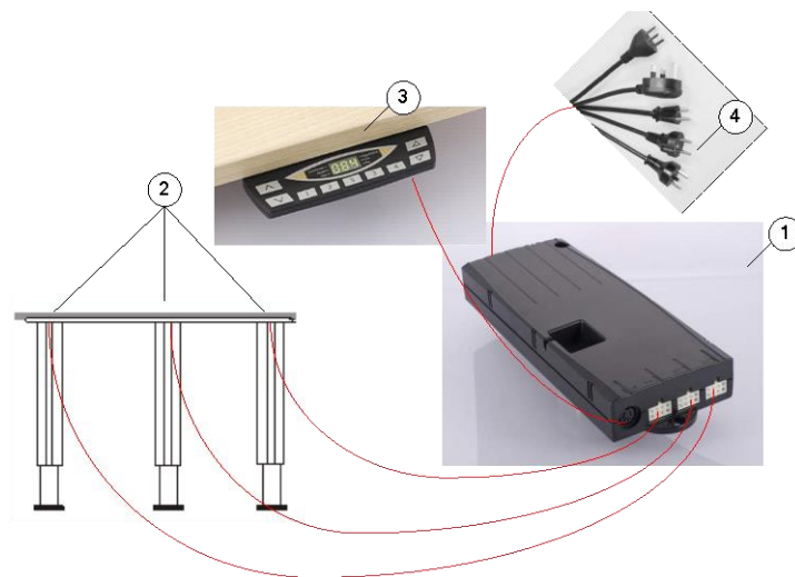
Figure 4: Configuration example
