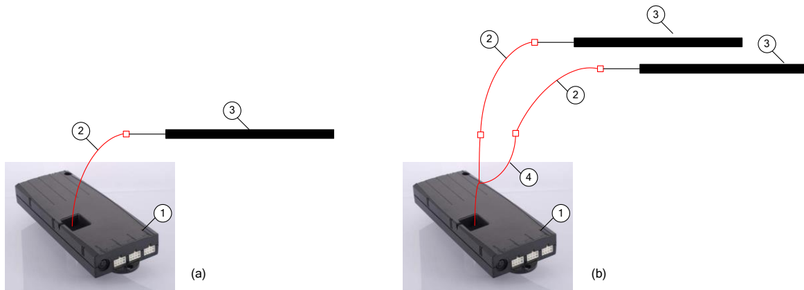
Figure 6: connection of (a) one squeeze line and (b) two squeeze lines
