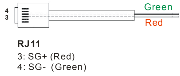
Figure 5 IFD6500 accessory RJ11 ↔ RS-485
